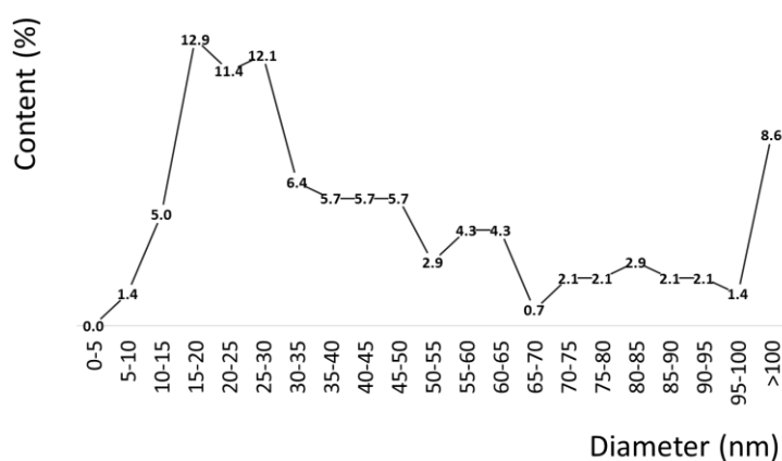
Fig. 3 Accumulated diameter distribution graph of the nanofibrils
