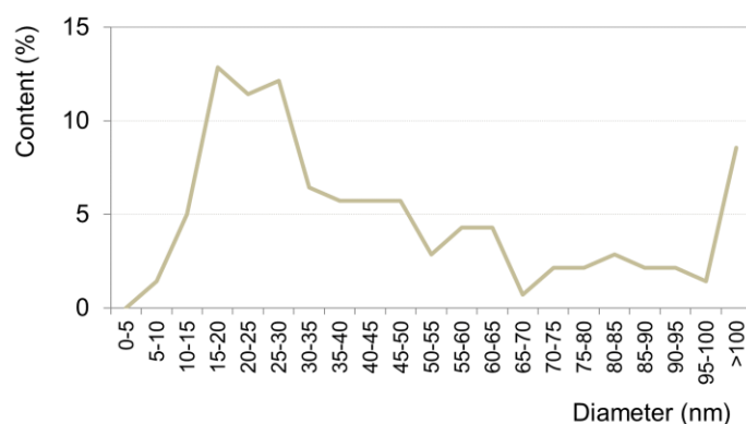
Fig. 3 Accumulated diameter distribution histogram of the nanofibrils
