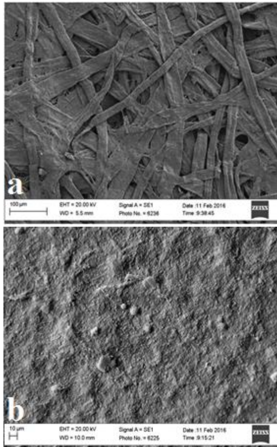
Fig. 11 Scanning electron microscopy images of the (a) uncoated paper (control) and (b) hybrid coating layer
