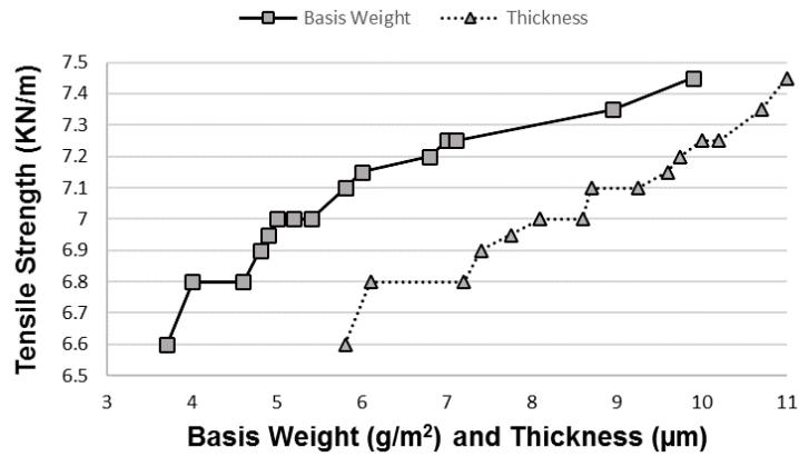
Fig. 7 Correlation between tensile strength of coated papers and basis weight and thickness of NFC layer
