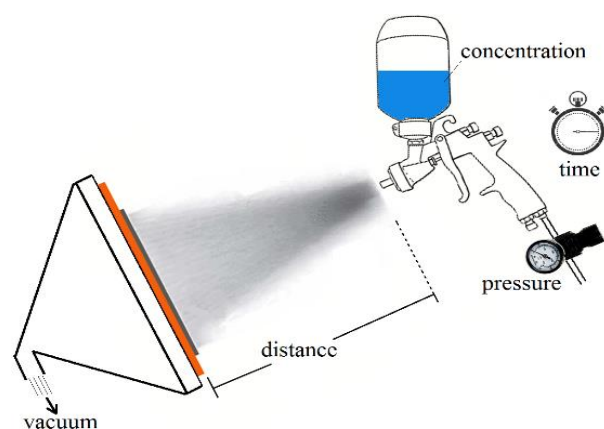
Fig. 1 Scheme of the experimental procedure used to coat the P&W paper substrates
