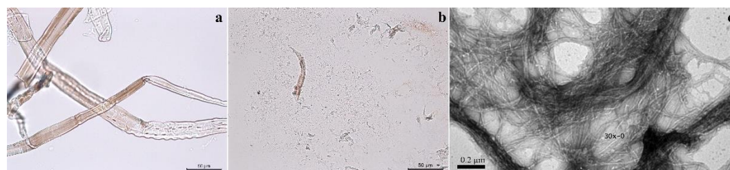
Fig. 2 Typical light microscopy (LM) images of the fibers:(a) before defibrillation; (b) after defibrillation; (c) typical transmission electron microscopy (TEM) micrograph of the nanofibrils derived from the defibrillation process
