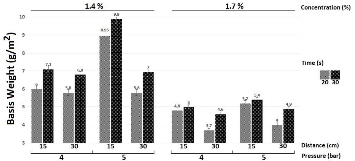
Fig. 4 Concentration, pressure, distance and time of spray impacts on basis weight of coated papers.
